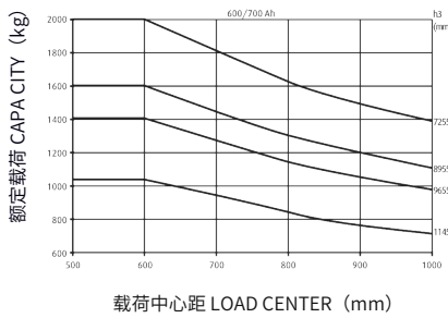
R20-L-负载曲线CAPACITY CHART (mm) 起升高度LIFT HEIGHT (mm)
